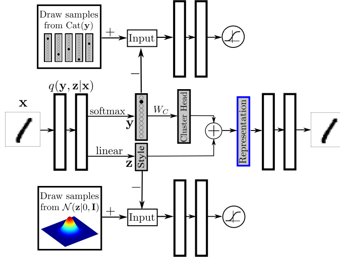
Figure 10: Dimensionality reduction with adversarial autoencoders: There are two separate adversarial networks that impose Categorical and Gaussian distribution on the latent representation. The final n dimensional representation is constructed by first mapping the one-hot label representation to an n dimensional cluster head representation and then adding the result to an n dimensional style representation. The cluster heads are learned by SGD with an additional cost function that penalizes the Euclidean distance between of every two of them.
