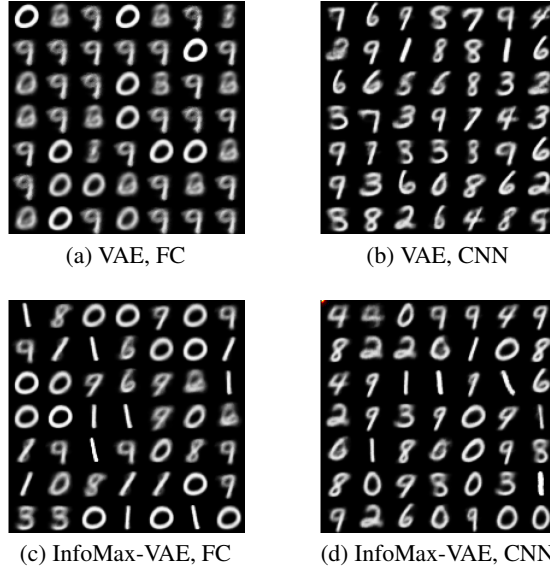
Figure 3: Generated samples by vanilla VAEs and InfoMax-VAE trained on MNIST dataset; (a)-(b) samples generated by vanilla VAE using FC and convolutional NNs, (c)-(d) samples of the proposed autoencoder, InfoMax-VAE, using similar architectures.
