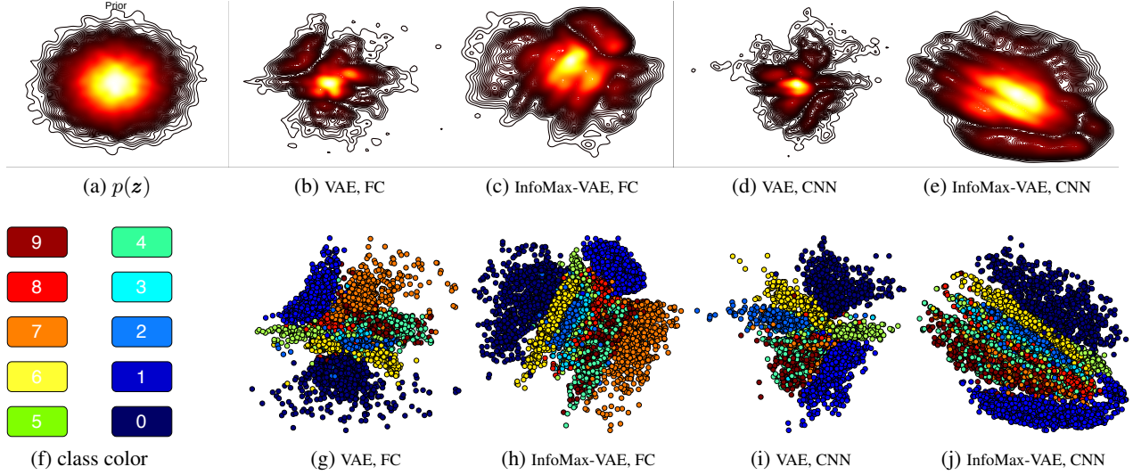
Figure 2: Comparing the prior p(\mathbf{z}) and the aggregated posterior q_\phi(\mathbf{z}) achieved by vanilla VAEs and InfoMax-VAE on MNIST dataset; (a) the prior p(\mathbf{z}) which is defined to be 2-D standard Gaussian distribution; (b)(c) aggregated posterior q_\phi(\mathbf{z}) of VAE and InfoMax-VAE with FC NNs; (d)(e) aggregated posterior q_\phi(\mathbf{z}) of VAE and InfoMax-VAE with CNN; (f) color of each class; (g)(h) latent codes of VAE and InfoMax-VAE with FC NN; (i)(j) latent codes of VAE and InfoMax-VAE with CNN.
