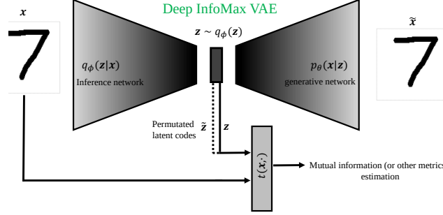
Figure 1: Architecture of InfoMax-VAE, a family of VAEs which encourages VAEs to learn useful high-level representations of data, the top networks can be convolutional or FC NNs. The bottom network ( t(\mathbf{x}, \cdot) ) is an MLP which estimates the mutual information between inferred latent representations \mathbf{z} and input data \mathbf{x} . Or, it can estimate any other strict divergence/distance between joint q_\phi(\mathbf{x}, \mathbf{z}) and the marginals q(\mathbf{x}), q_\phi(\mathbf{z}) .
