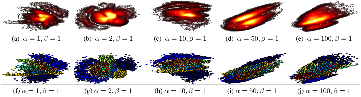
Figure 7: The aggregated posterior q_\phi(\mathbf{z}) (first row) with their associated latent codes (second row). Varying \alpha with fixed \beta .
