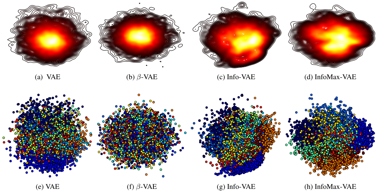
Figure 4: Comparing the prior p(\mathbf{z}) and the aggregated posterior q_\phi(\mathbf{z}) of Pixel VAEs, Pixel \beta -VAE, and Pixel InfoMax-VAE on binarized MNIST dataset; (a) vanilla Pixel VAE, (b) Pixel \beta -VAE, (c) Pixel Info-VAE, (d) Pixel InfoMax-VAE (e)-(h) the latent codes generated by their associated models; latent codes of each categories are painted with different colors. We see that Pixel InfoMax-VAE outperforms three other models as it pushes the learned features of each classes to be assembled in a more meaningful fashion.
