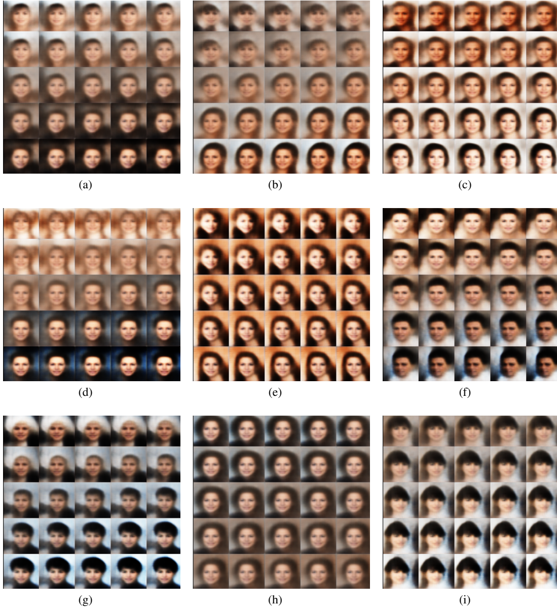
Figure 9: Qualitative results for CelebA dataset. In each case, 10% of the latent codes are varying from -4 to 4, and the rest of them are fixed.
