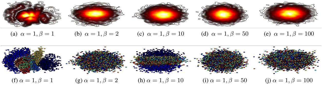
Figure 8: The aggregated posterior q_\phi(\mathbf{z}) (first row) with their associated latent codes (second row). Varying \beta with fixed \alpha .
